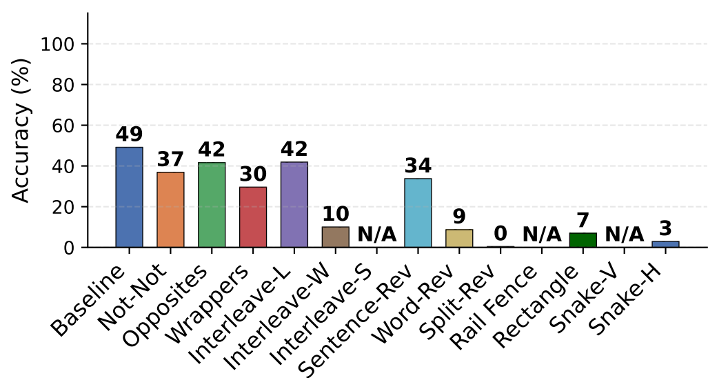
DSR1-Llama-70B
