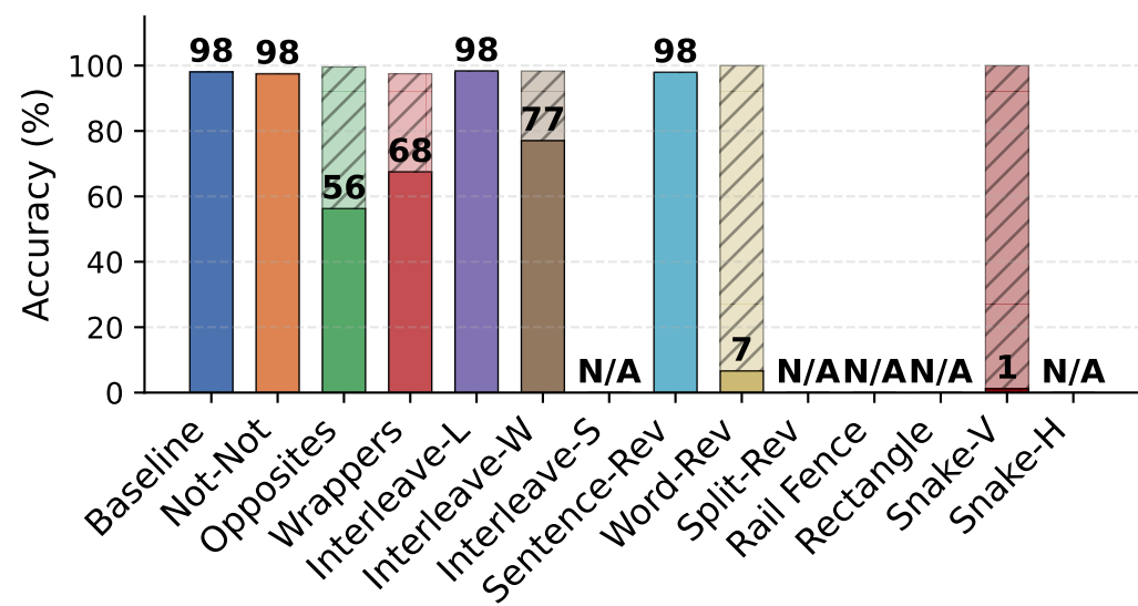
GPT-OSS-120B
