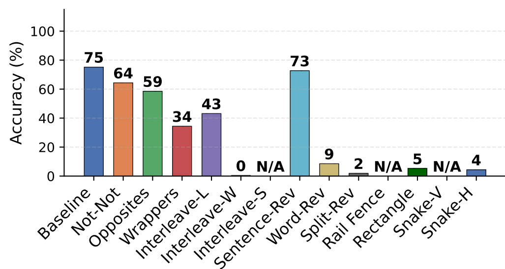
Nemotron-7B
